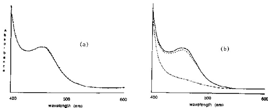
Figure 9. Absorption spectrum of \text{Pt(dpphen)(ecda)} , 3e , after photolysis in the presence of (a) DMA and (b) ONB.
