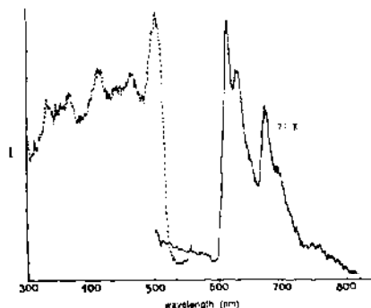
Figure 2. Excitation (---) and emission (—) spectra of \text{Pt}(\text{dmbpy})(\text{mnt}) , 1c, in the solid state at 77 K.
