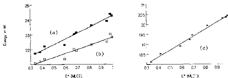
Figure 1. Correlation between transition energy and E^*_{\text{MLCT}} for (a) \text{Pt}(\text{dmbpy})(\text{ecda}) , (b) \text{Pt}(\text{dpphen})(\text{ecda}) and (c) \text{Pt}(\text{dpphen})(\text{mnt}) .
